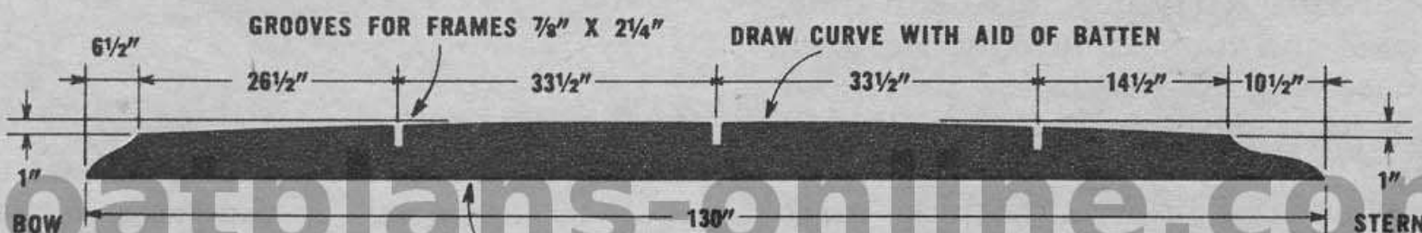
BACK BONE OF JIG 2X6 STRAIGHT DRY PLANK
